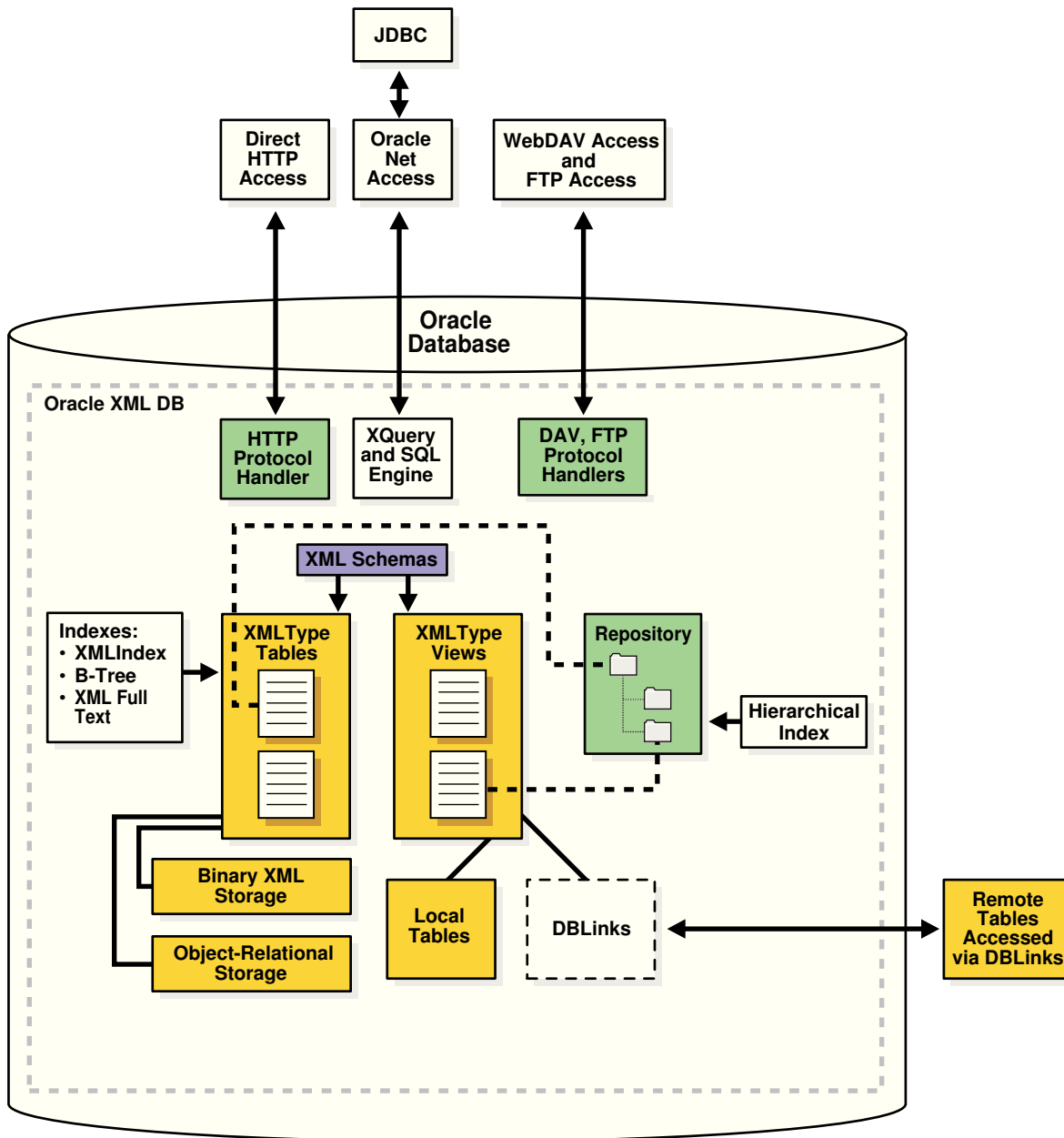
Figure 1-3 XMLType Storage
